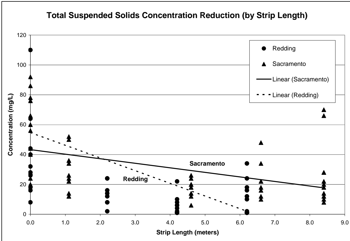
Figure 4. TSS Concentration as a Function of Strip Length (Lines indicate trend, not performance)
