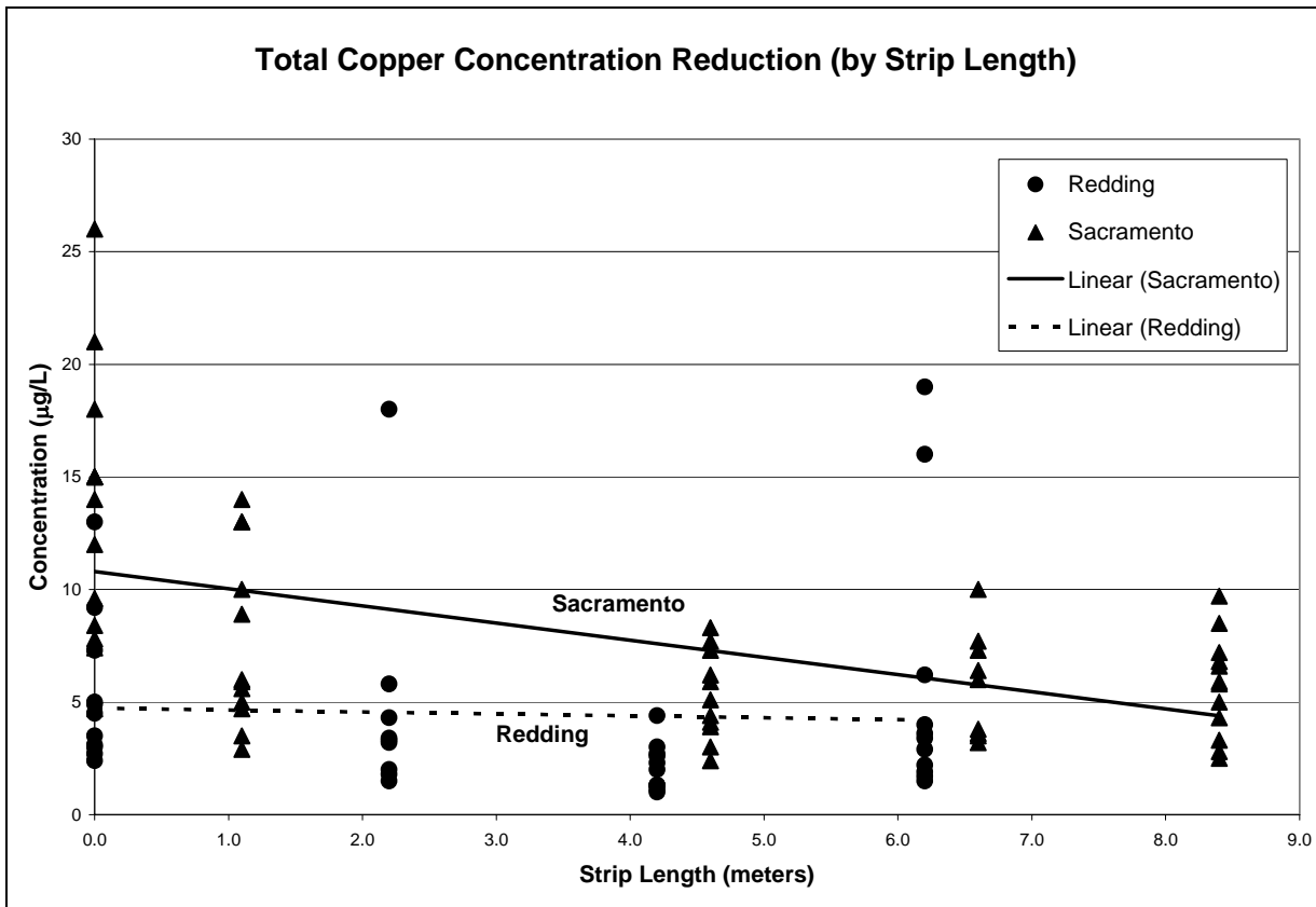
Figure 5. Total Copper Concentration as a Function of Strip Length (Lines indicate trend, not performance)
