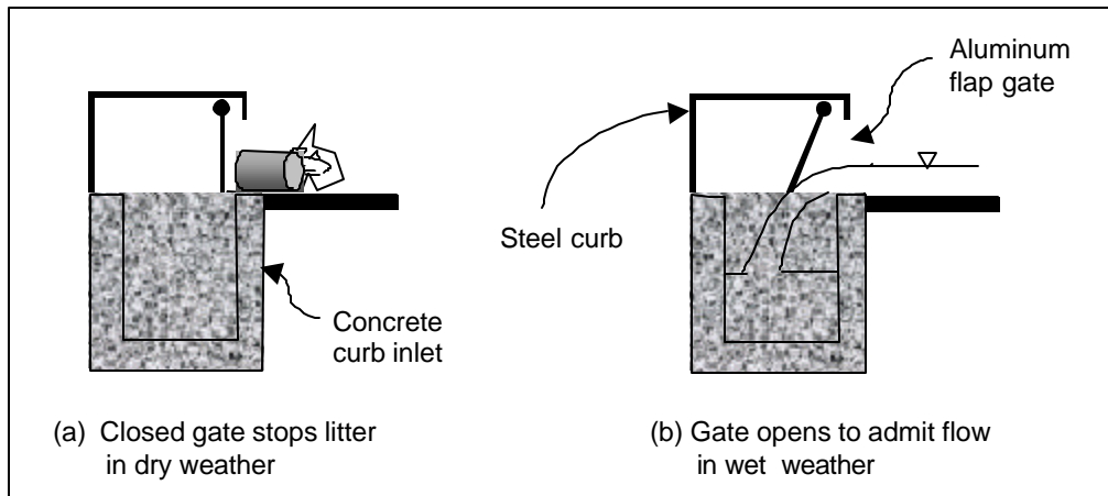
Figure 3 Litter Inlet Deflector Schematic
