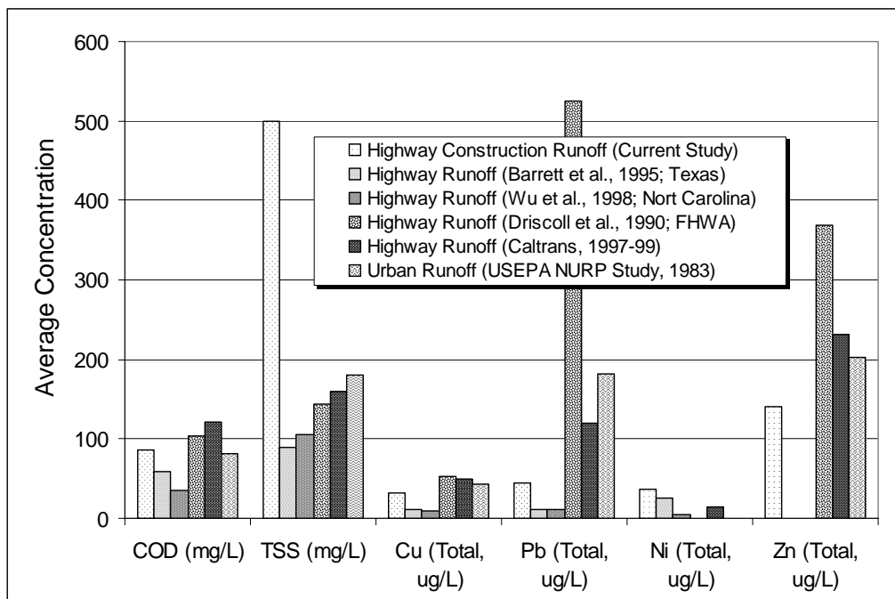
FIGURE 3 Comparison of Construction Site and Highway Storm Water Runoff Concentration for Selected Constituents
