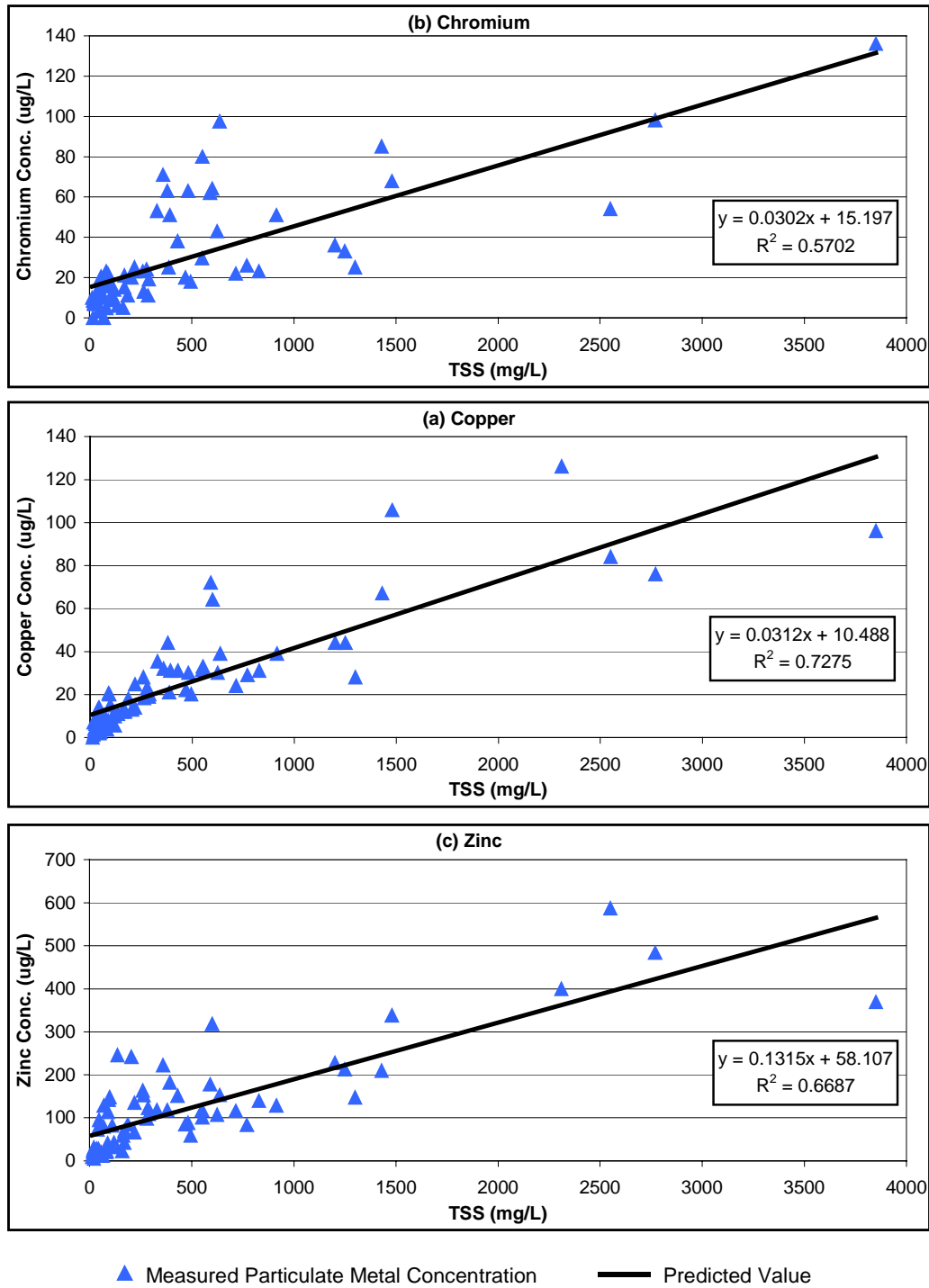
FIGURE 5 Correlation Between TSS and Particulate Metal for Chromium, Copper, and Zinc
